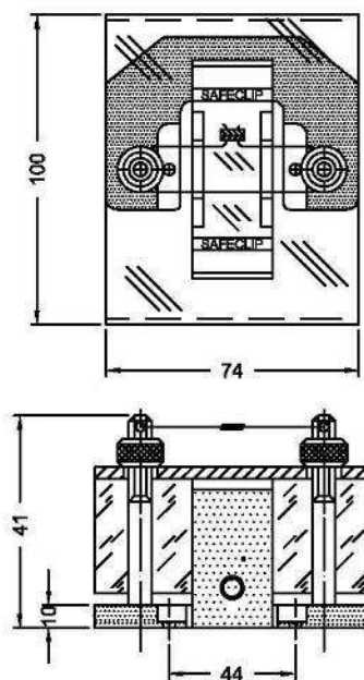
SINGLE FUSE SEALING BLOCK
